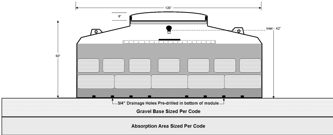
View 1: Cross Section, Length
